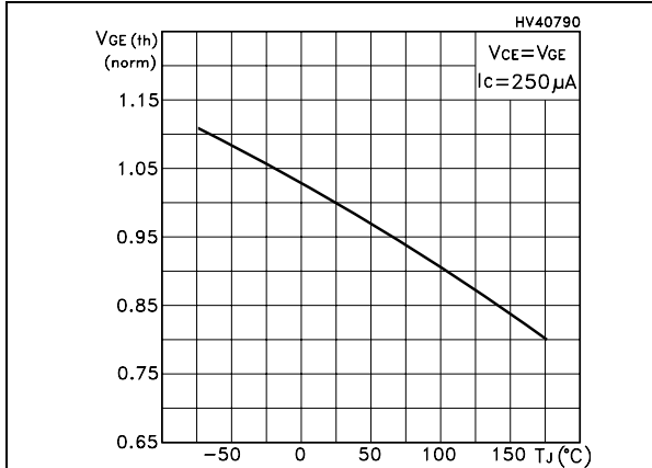
Figure 8. Normalized gate threshold voltage vs temperature
